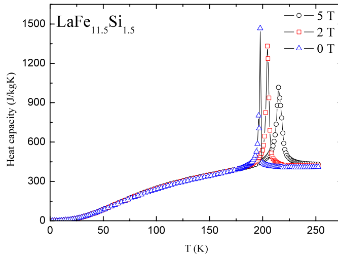
Figure 6. The heat capacity as a function of temperature and magnetic field from 2 to 252 K. The solid lines are guides for the eye.
